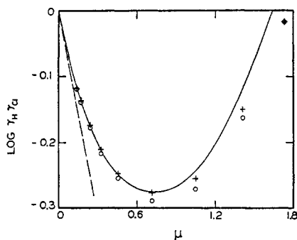
FIG. 9. Comparison of the activity coefficients of electrolytes in sodium chloride solutions at 25°C. Smooth curve, \log \gamma_{\text{H}}\gamma_{\text{Cl}} ; O, \log \gamma_{\text{H}}\gamma_{\text{OH}}/a_{\text{H}_2\text{O}} ; +, \log \gamma_{\text{H}}\gamma_{\text{Ac}}/\gamma_{\text{HAc}} .
